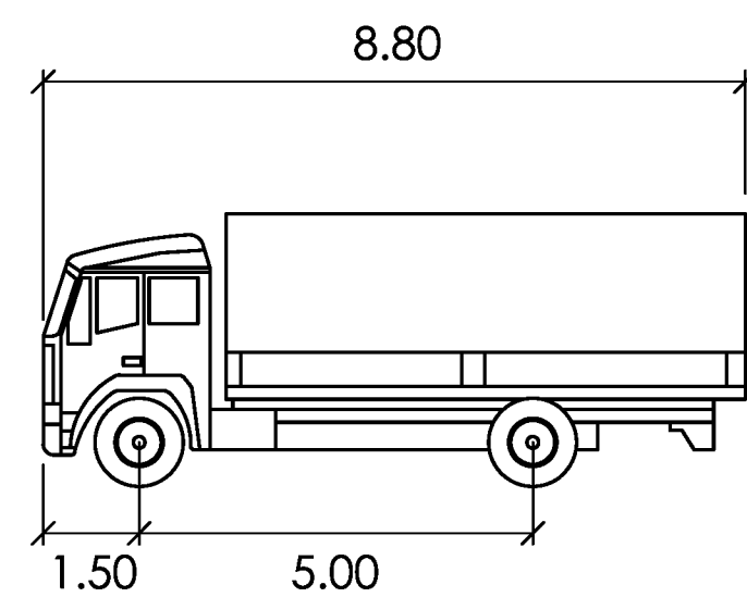
Medium Ridged Vehicle (MRV)
